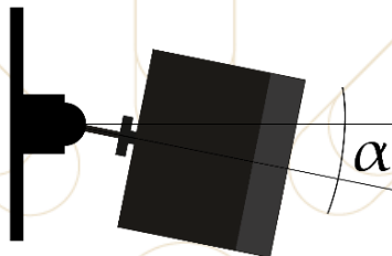
Figure 17 - Base station mount with angle
