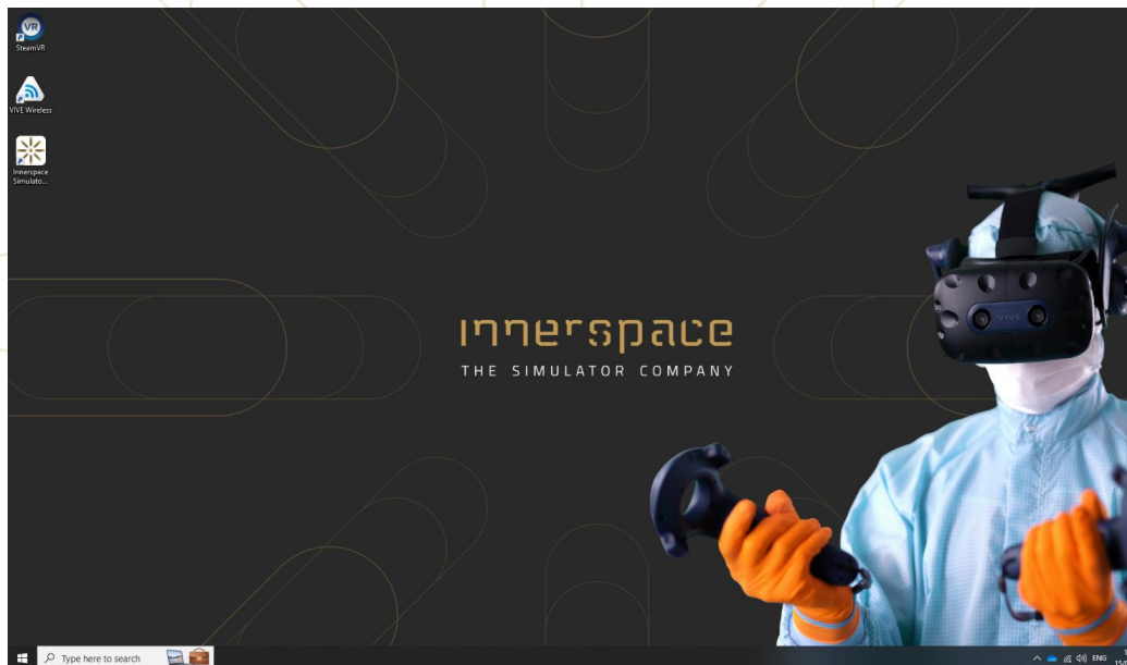
Figure 23 - Windows Desktop
