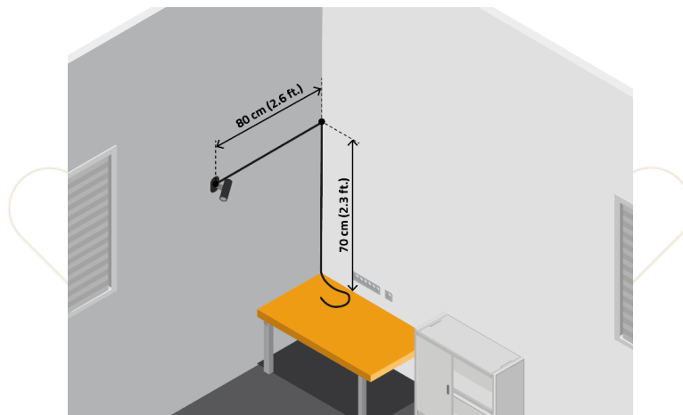
Figure 6 - HTC wireless link box mount option 1
