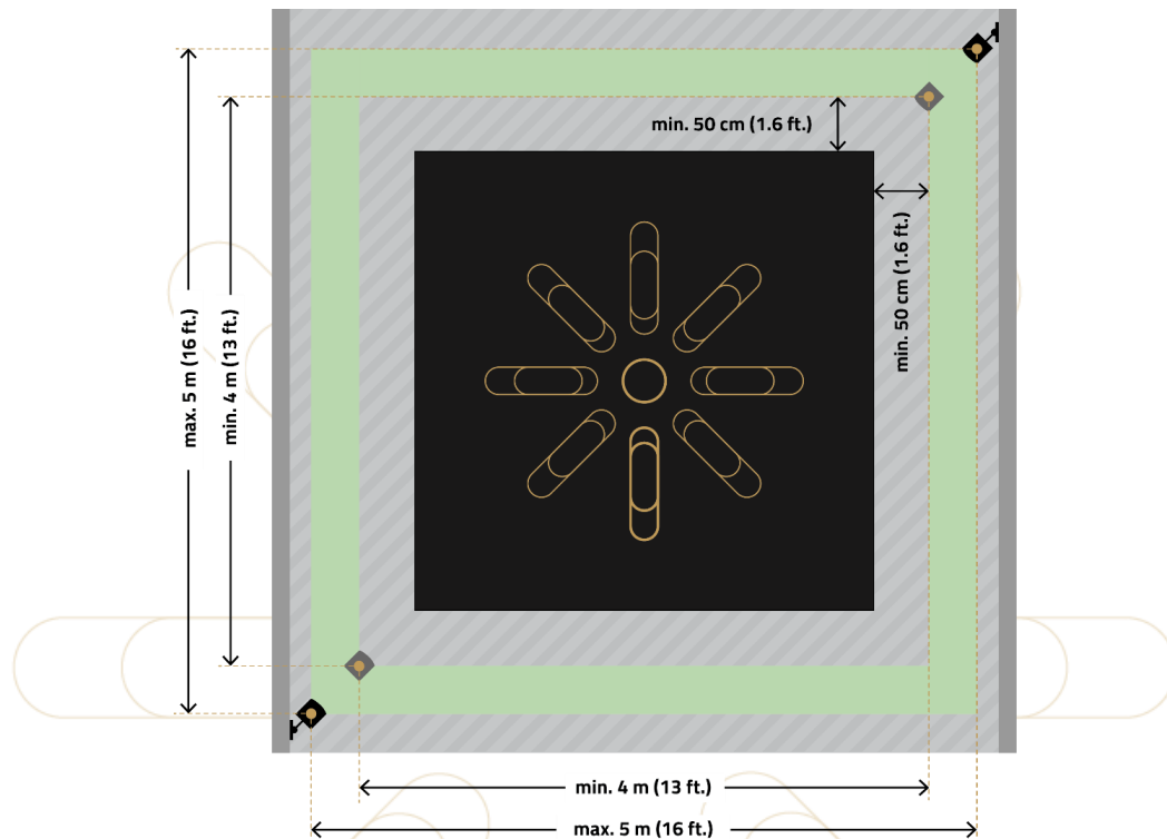
Figure 3 - Base station distance from a top-down view
